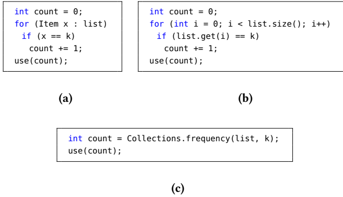
Figure 2. Java variations of array frequency count
